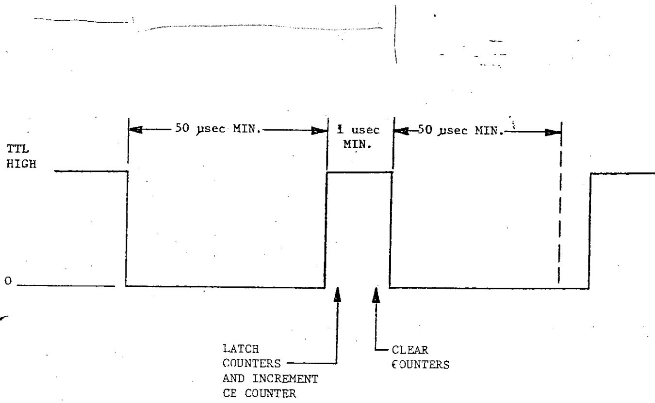
FIG. 4 COUNT ENABLE TIMING
